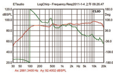
Frequency Response Curve
