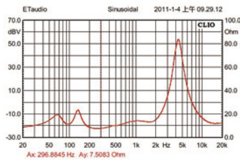
Impedance Curve
