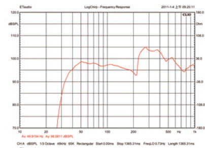
Frequency Response Curve
