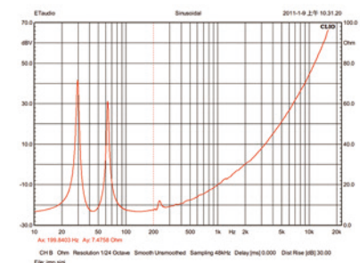
Impedance Curve
